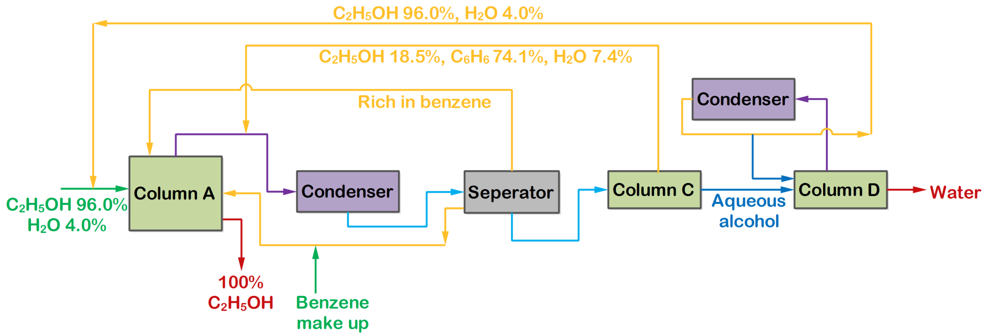
Figure: Manufacture of Absolute alcohol from 96% alcohol
